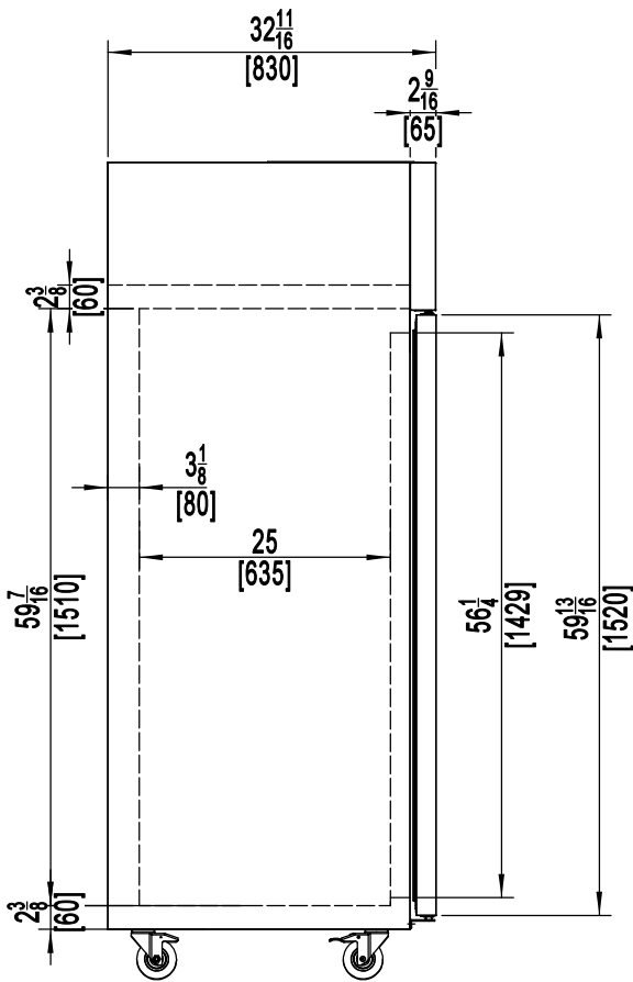
SIDE VIEW
